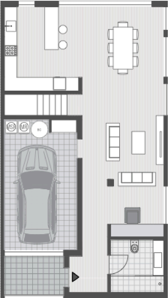
PISO 0 GROUND FLOOR 112 m 2
